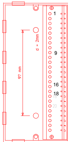
Montagesockel (LxBxH): 158x75x35mm Base (LxWxH): 158x75x35mm
